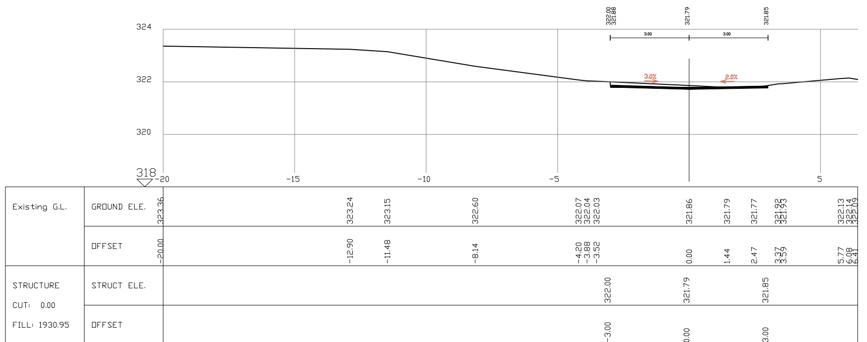
SECTION 7 St. 140 Road1
