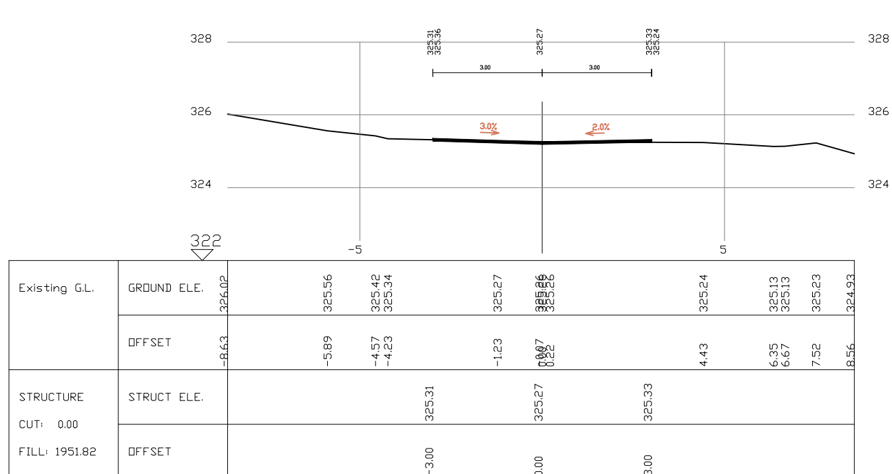
SECTION 11 St. 220 Road1
