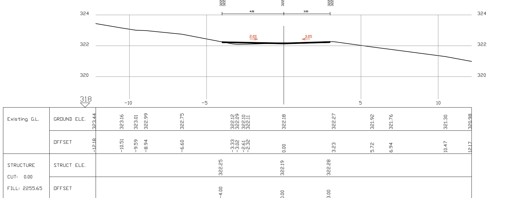
SECTION 8 St. 160 Road1
