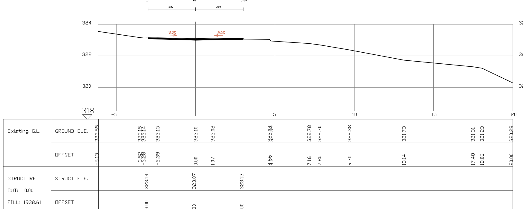
SECTION 9 St. 180 Road1
