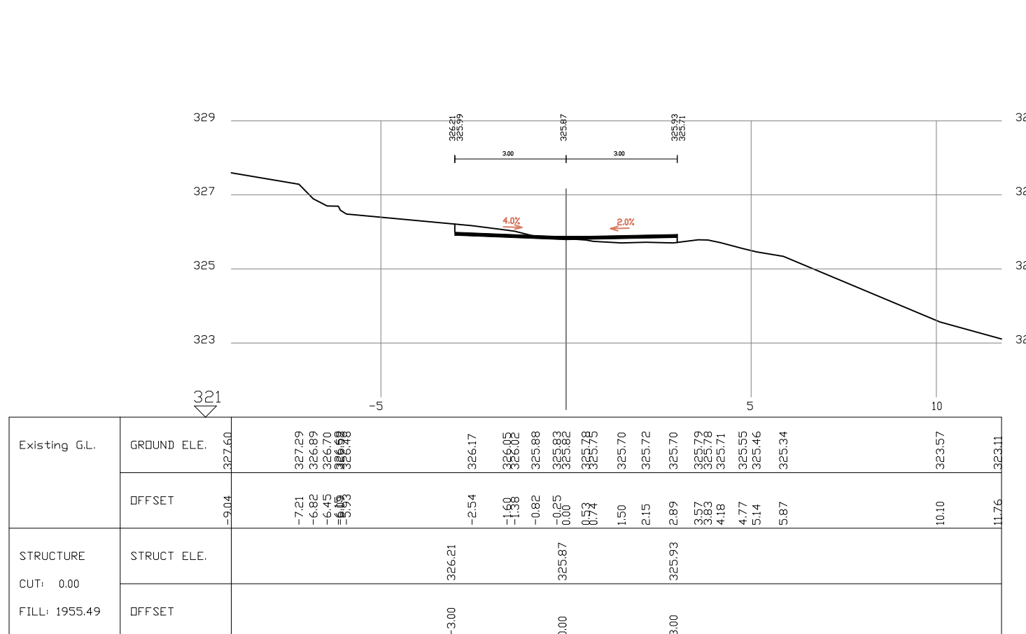
SECTION 13 St. 240.69 Road1
