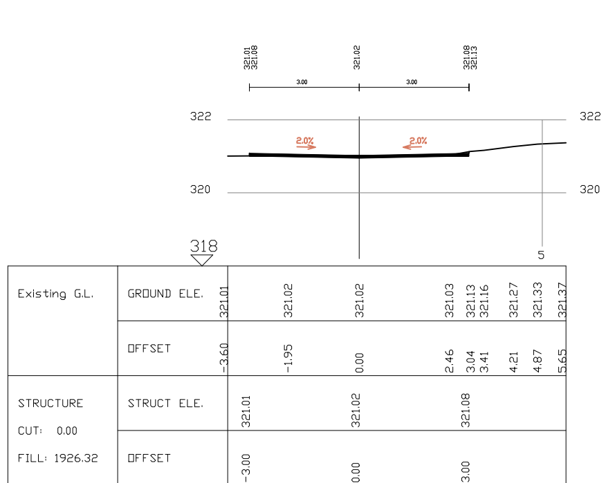
SECTION 4 St. 80 Road1
