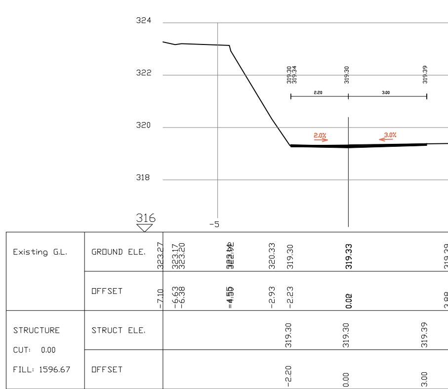
SECTION 0 St. 0 Road1
