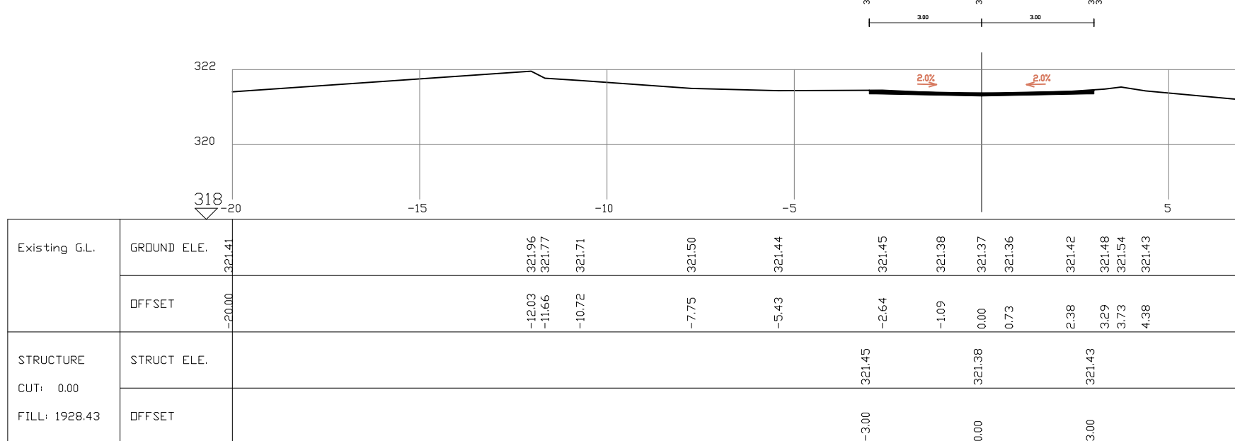
SECTION 6 St. 120 Road1
