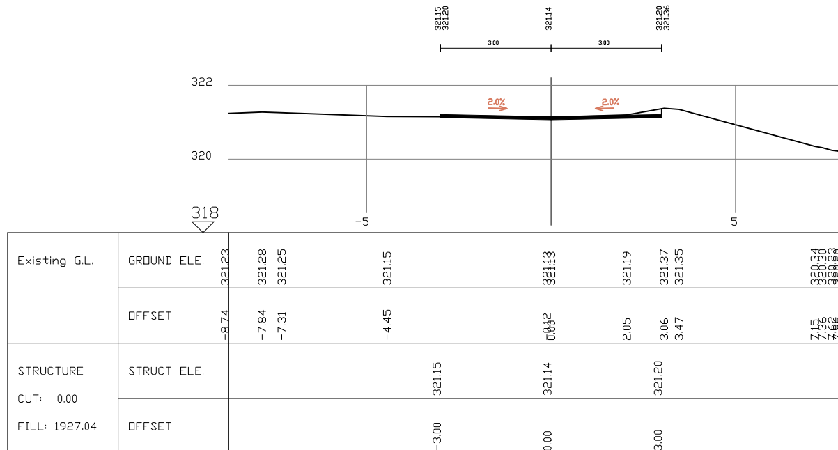
SECTION 5 St. 100 Road1
