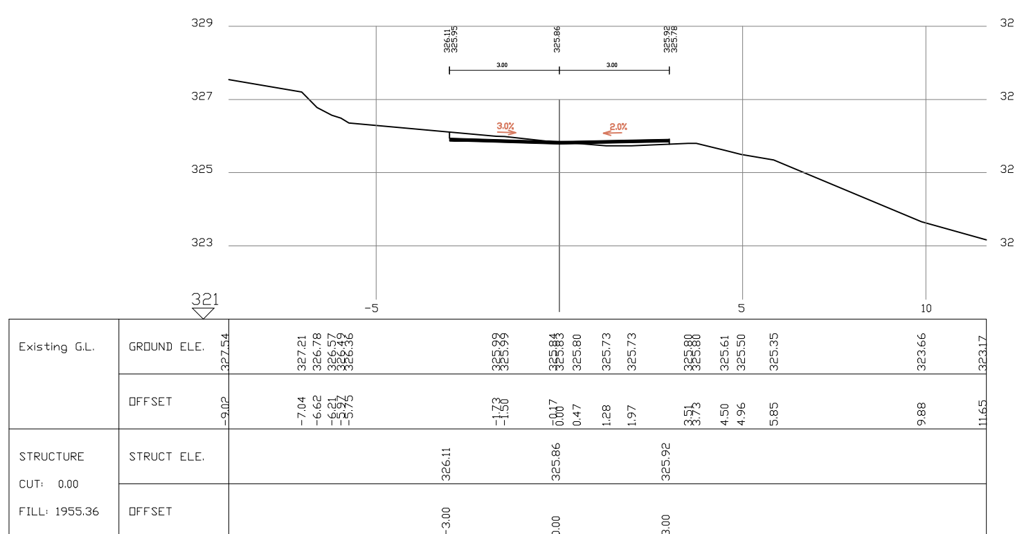
SECTION 12 St. 240 Road1
