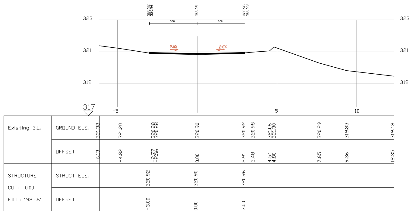
SECTION 3 St. 60 Road1
